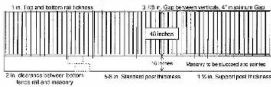
Elevation C: Combination Party Wall/Fence
