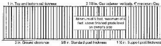
Elevation B: Wrought Iron Party Fence
