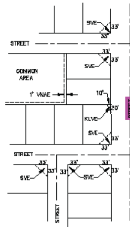
PLAN VIEW
